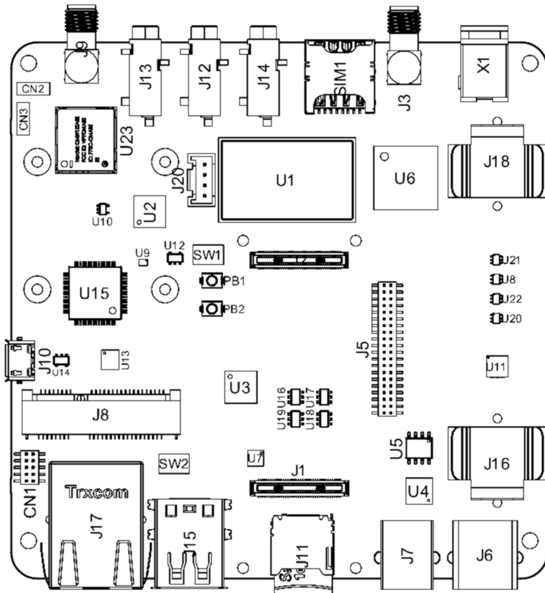
Board topology
