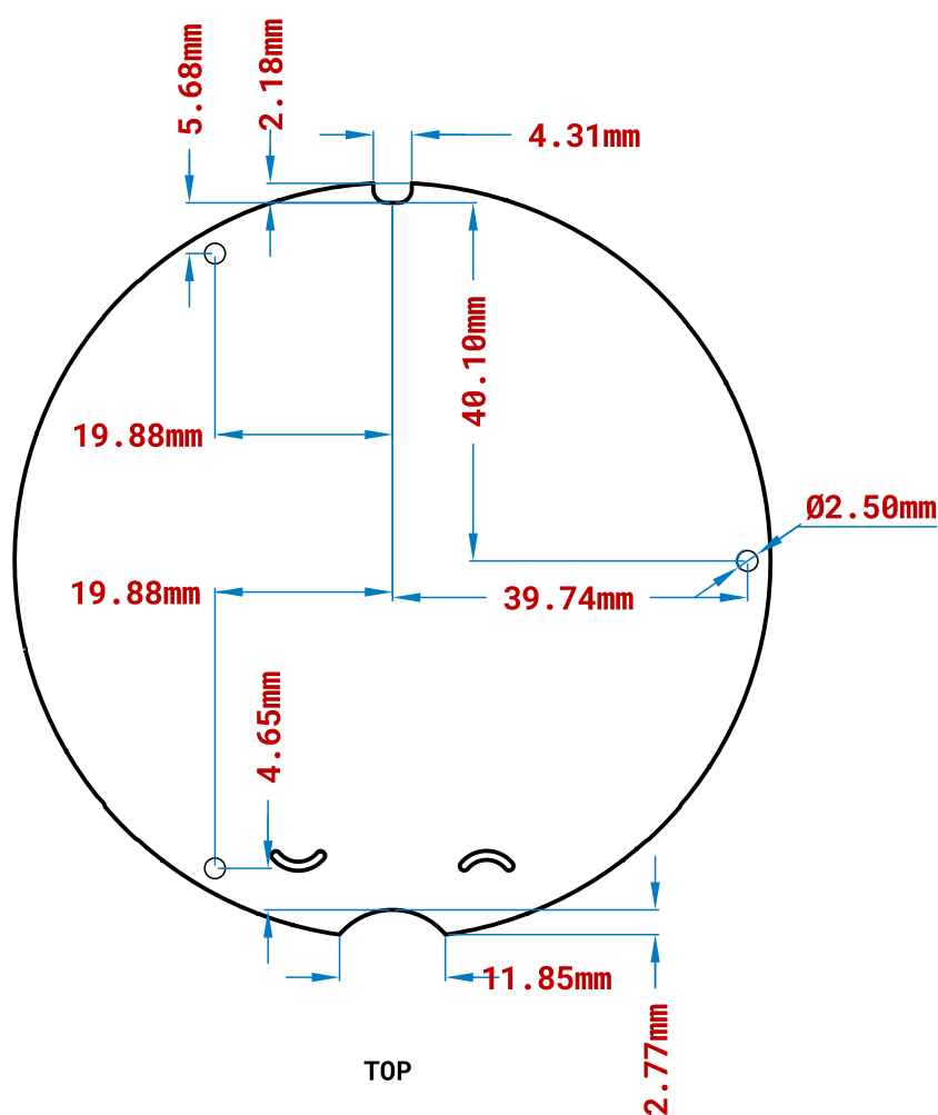
Mechanical view
